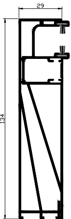
WNS 135 Duo Line
