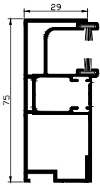
WNS 75 Duo Line
